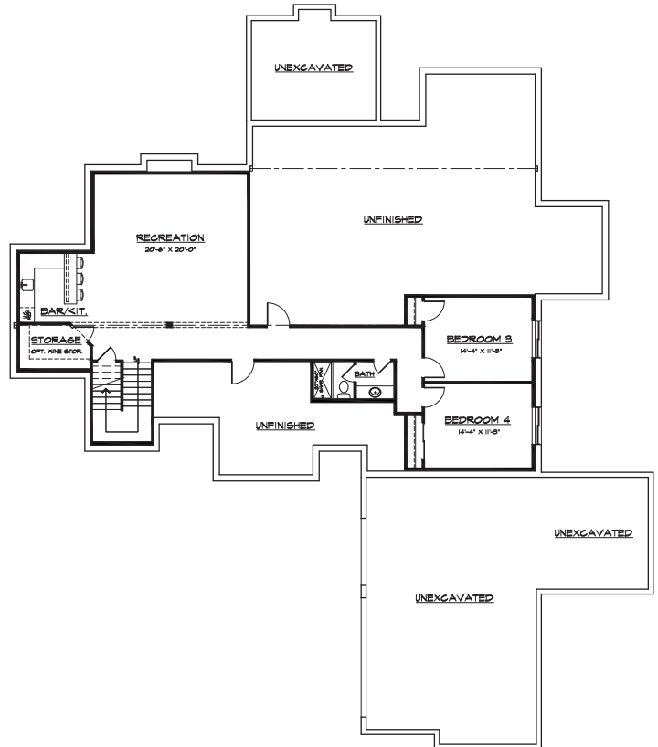
LOWER LEVEL 1,223 Sq. Ft.
