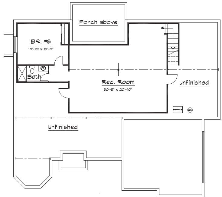
LOWER LEVEL 1,045 Sq. Ft.
