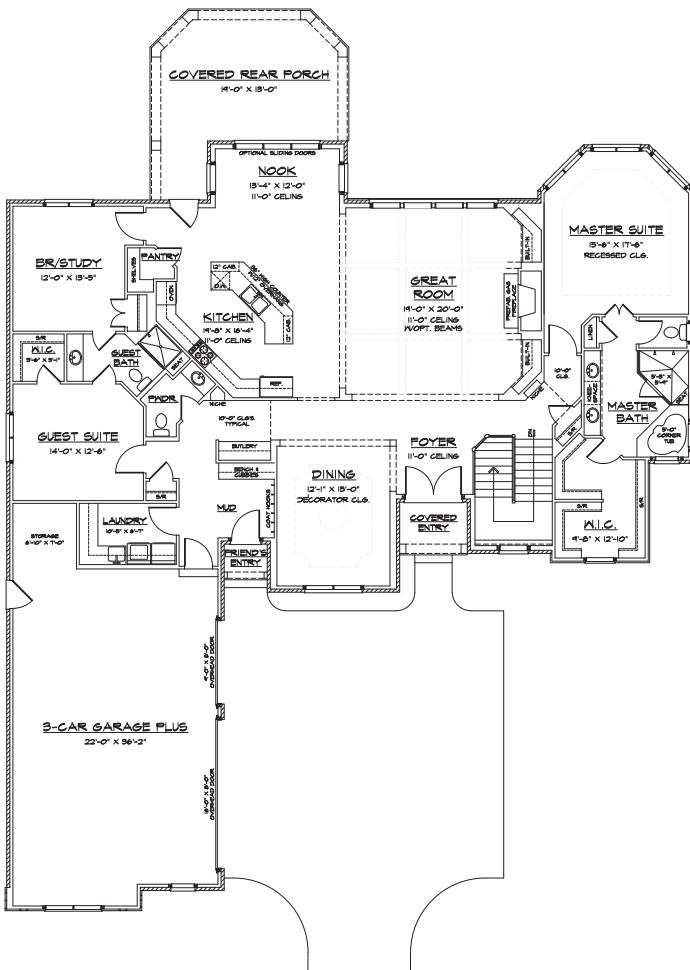
FIRST FLOOR 2,931 Sq. Ft.
